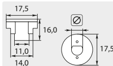
Coupling for shaft \varnothing 8 mm short
