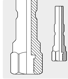
Plug KW : 1/4" F. SW 19. Polished stainless steel. For moulded handles. Plug for aluminium washer
