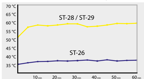
Surface temperature of the insulations ST-28, ST-29 and ST-26 at a water temperature of 90 °C.
